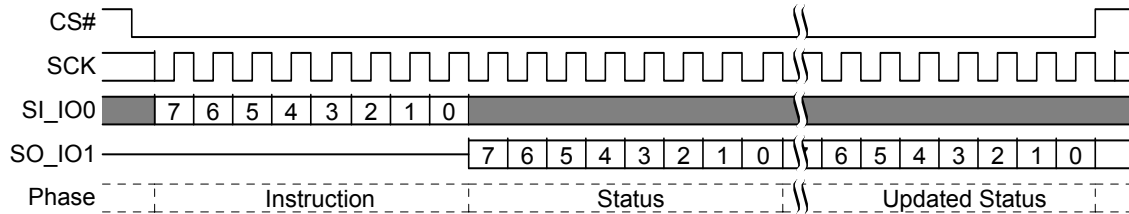
Figure 9.9 Read Status Register-1 (RDSR1) Command Sequence
